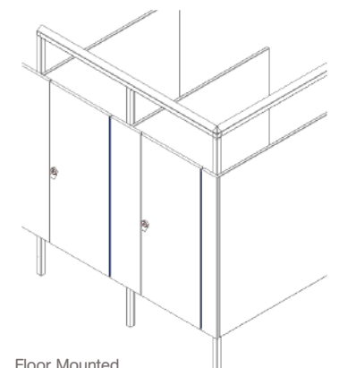
Floor Mounted Overhead Braced
